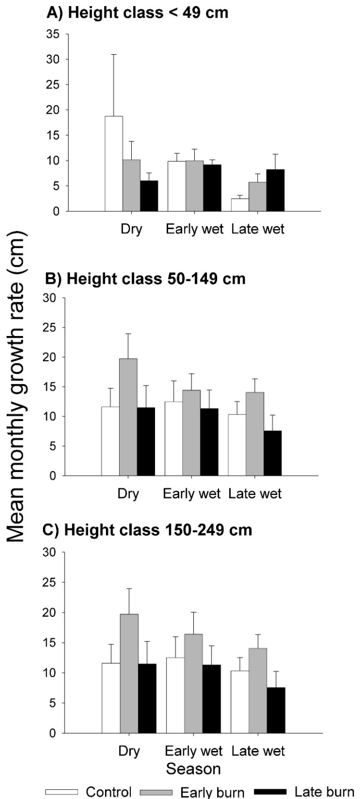
Figure 3. Mean monthly growth rates of Acacia sieberiana height classes, A , <49 cm; B , 50–149 cm; and C , 150–249 cm, during different seasons and treatments in Kidepo Valley National Park, Uganda. Error bars (SE) show variation among individuals of different height classes in 14 replicate blocks for each treatment. No significant treatment differences were found (one-way ANOVA tests). Seasons: dry (November–February), early wet (March–June), and late wet (July–October).
