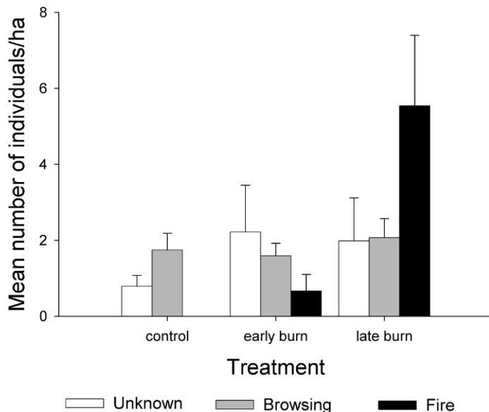
Figure 4. Causes of Acacia sieberiana mortality during 3 yr of experimental burning in Kidepo Valley National Park, Uganda. Error bars (SE) show variation among 14 replicate blocks for each treatment.
