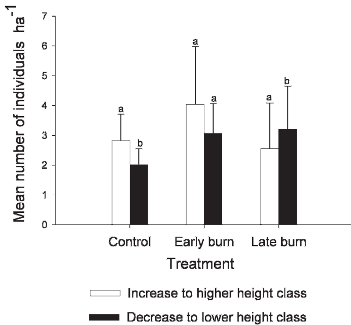
Figure 2. Height class changes in Acacia sieberiana trees in different treatments during 3 yr of experimental burning in Kidepo Valley National Park, Uganda. Error bars (SE) show variation among 14 replicate blocks for each treatment. Different letters indicate significant differences between numbers of trees, within a treatment, that increase to higher height classes and the number of trees that are reduced to lower height classes.
