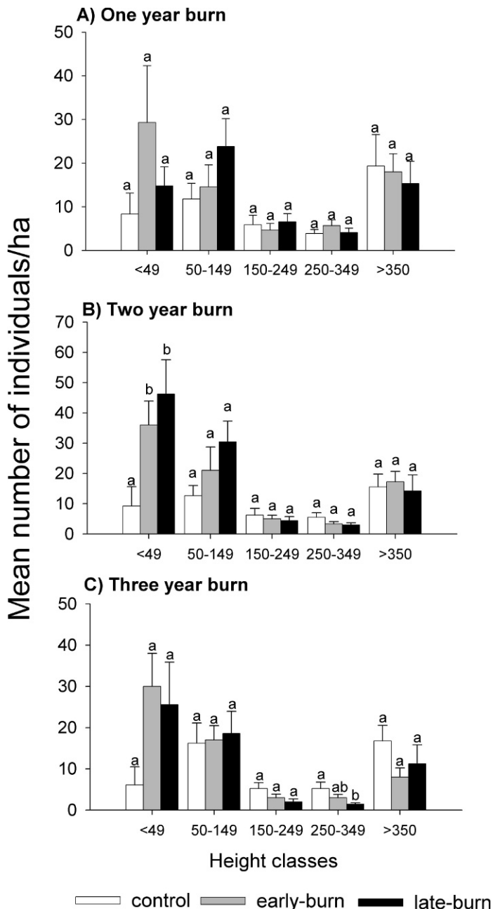
Figure 1. Tree height class distribution of Acacia sieberiana in A , 1-yr burn; B , 2-yr burn; and C , 3-yr burn during experimental burning in Kidepo Valley National Park, Uganda. Error bars (SE) show variation among 14 replicate blocks for each treatment. Different letters indicate a significant difference among treatments within height class, one-way ANOVA and Bonferroni post hoc test.
